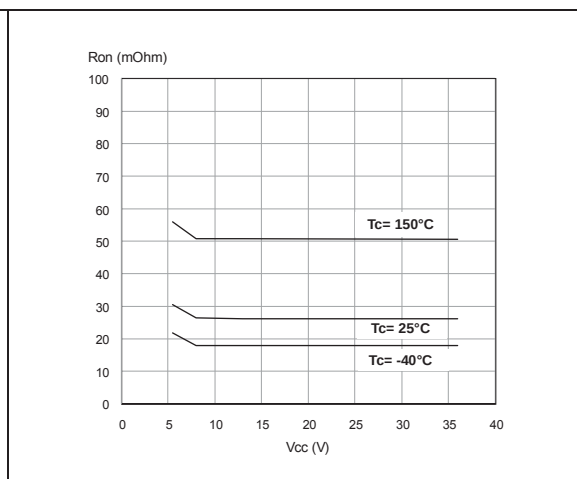
Figure 19. On-state resistance vs V_{CC}
